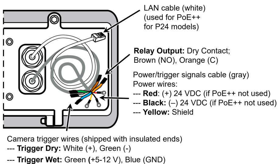
Figure 8. Cable Details
