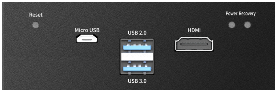
Figure 3. Front Panel
