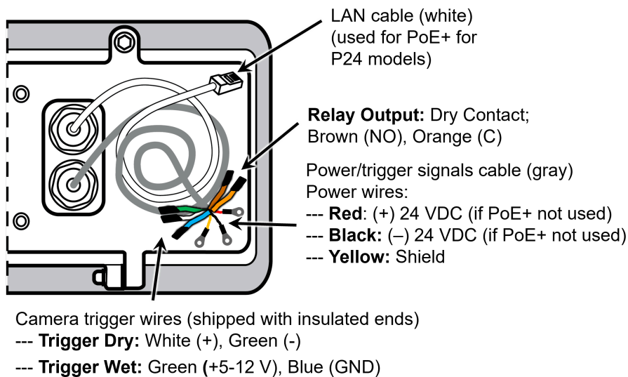
Figure 9. Cable Details
